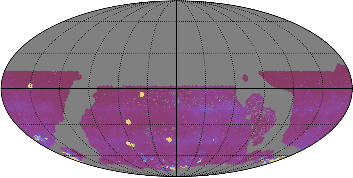
ddf_acor_sf20_lsf30_lsr10_v3.4_10yrs WFD iz bands: 75th Percentile Intranight Timespan
