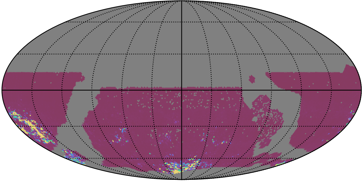
ddf_acor_sf20_lsf30_lsr10_v3.4_10yrs WFD gr bands: 75th Percentile Intranight Timespan
