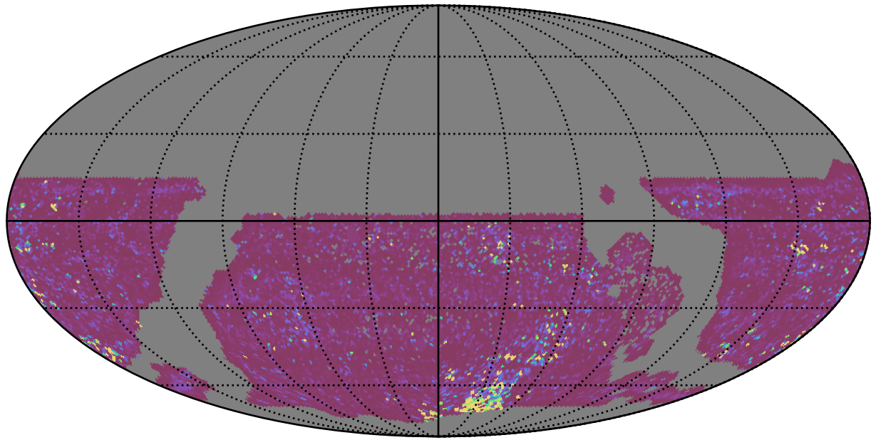
ddf_acor_sf20_lsf30_lsr10_v3.4_10yrs WFD g band: 75th Percentile Intranight Timespan
