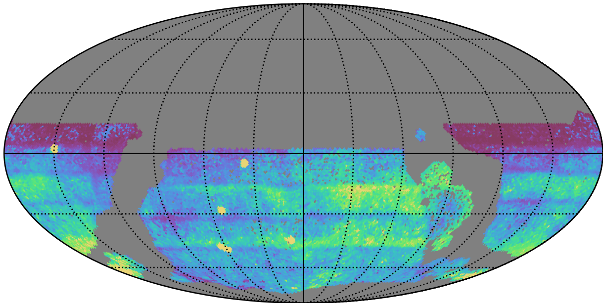
ddf_acor_sf20_lsf30_lsr10_v3.4_10yrs WFD all bands: 75th Percentile Intranight Timespan
