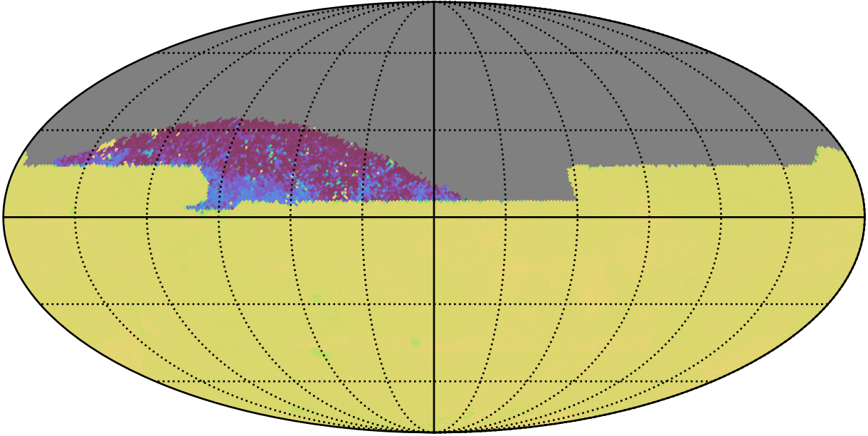
ddf_acor_sf20_lsf30_lsr10_v3.4_10yrs All sky zy bands: 75th Percentile Intranight Timespan
