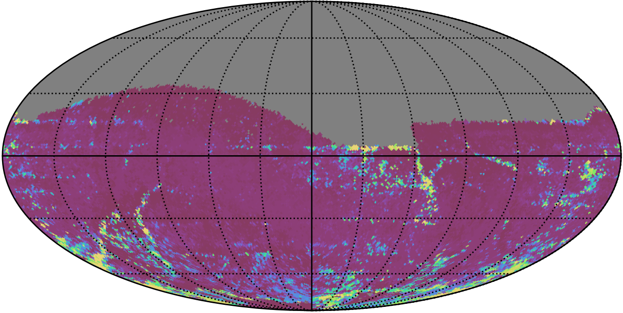
ddf_acor_sf20_lsf30_lsr10_v3.4_10yrs All sky z band: 75th Percentile Intranight Timespan
