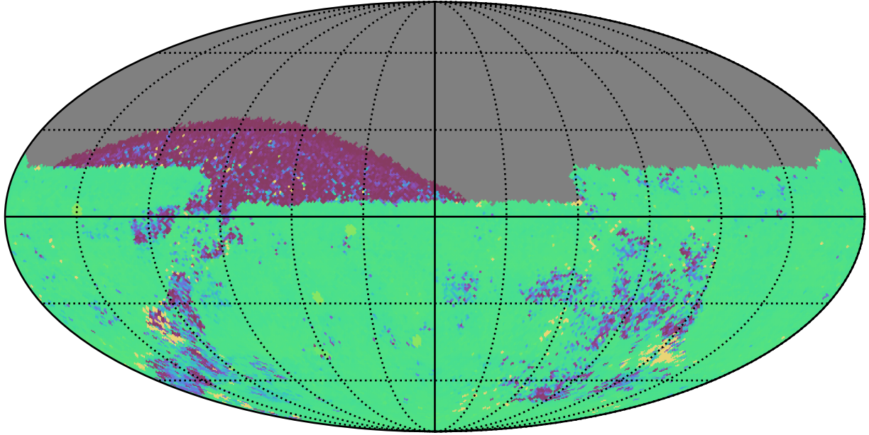
ddf_acor_sf20_lsf30_lsr10_v3.4_10yrs All sky ug bands: 75th Percentile Intranight Timespan
