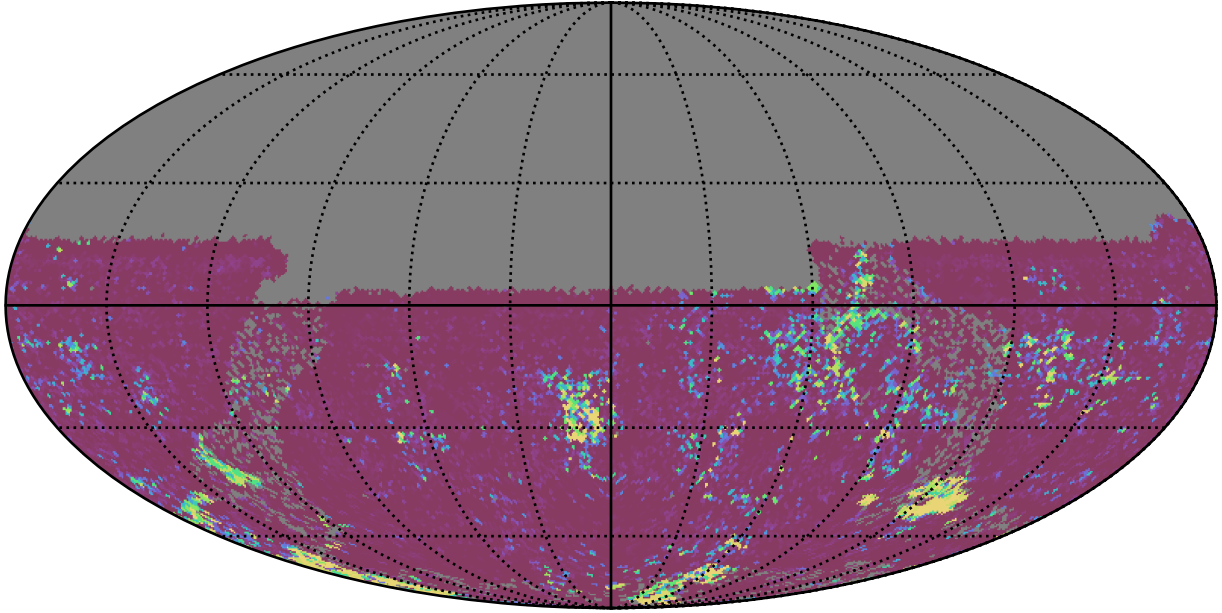
ddf_acor_sf20_lsf30_lsr10_v3.4_10yrs All sky u band: 75th Percentile Intranight Timespan
