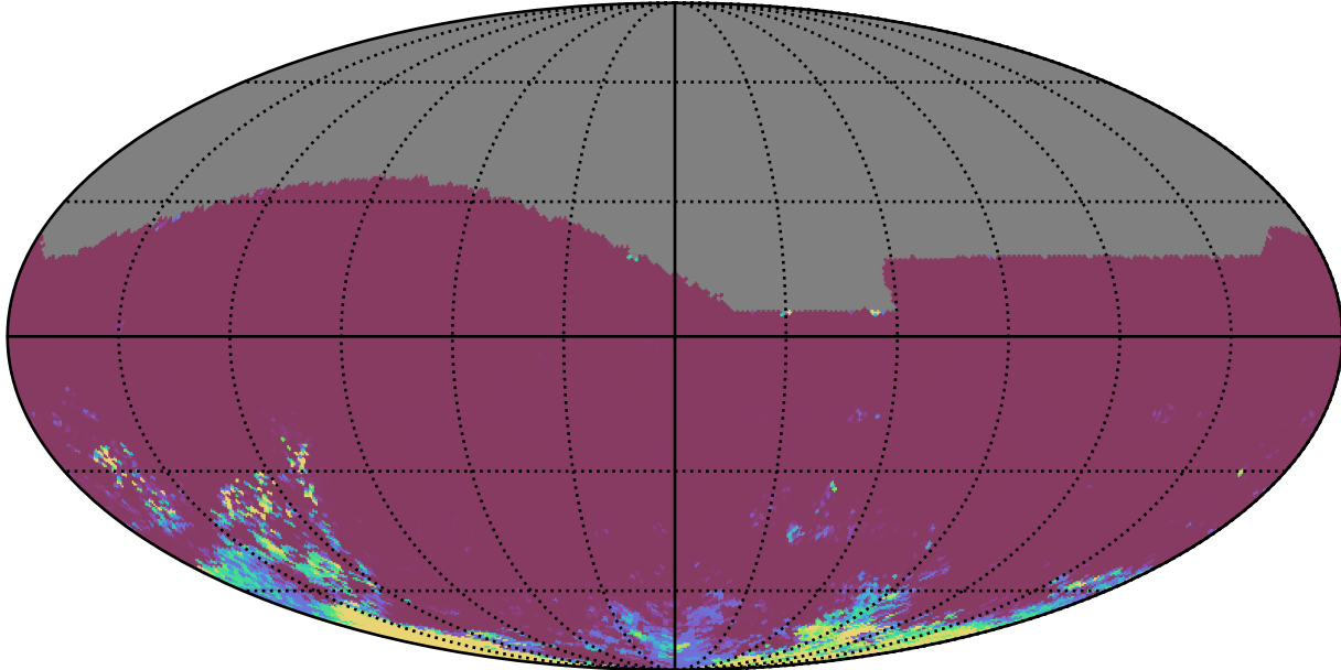
ddf_acor_sf20_lsf30_lsr10_v3.4_10yrs All sky ri bands: 75th Percentile Intranight Timespan
