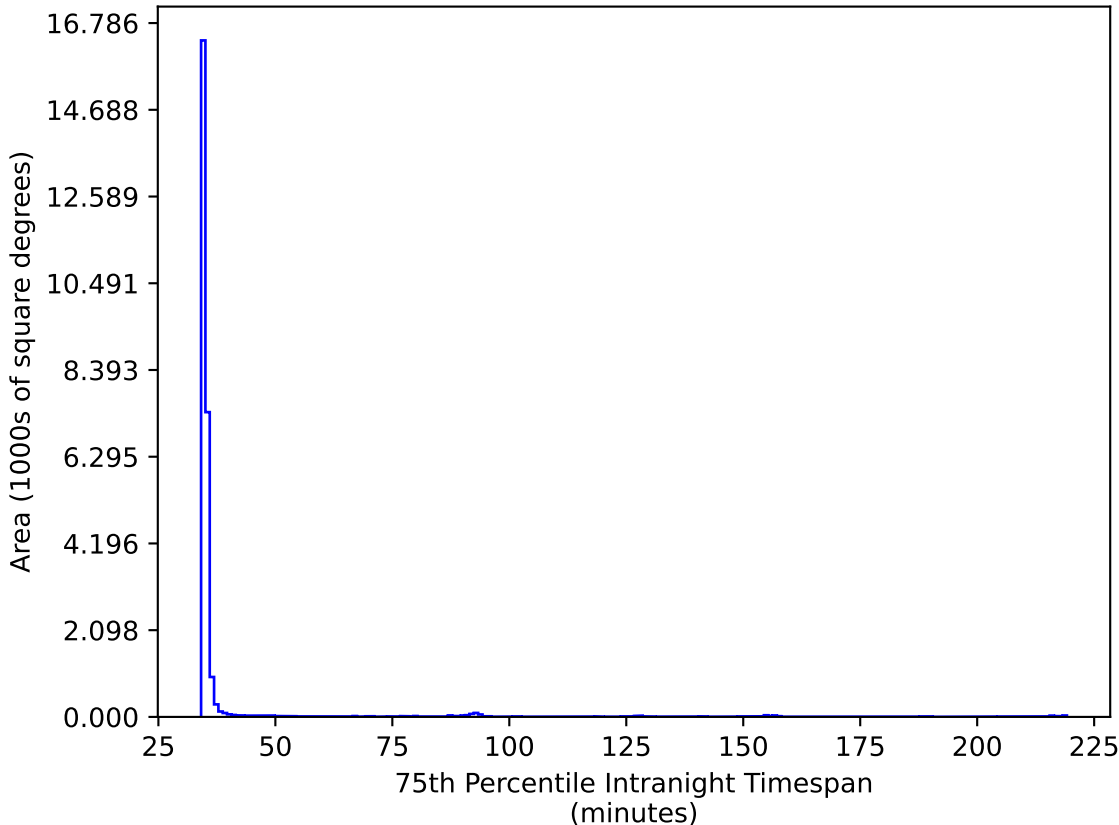
ddf_acor_sf20_lsf30_lsr10_v3.4_10yrs All sky ri bands: 75th Percentile Intranight Timespan
