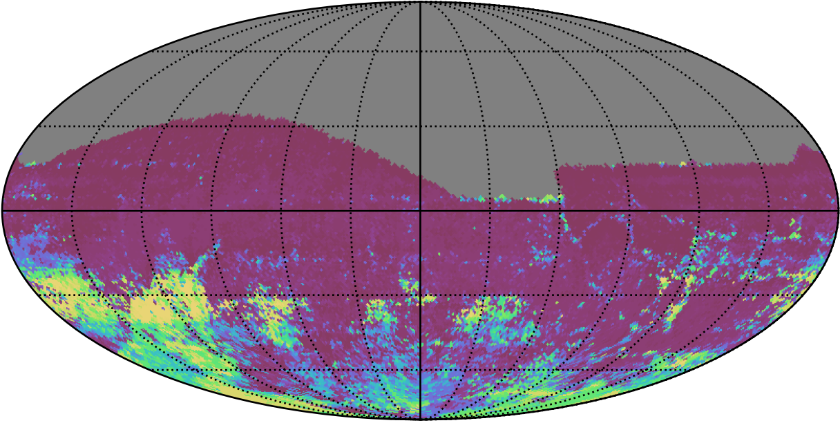
ddf_acor_sf20_lsf30_lsr10_v3.4_10yrs All sky r band: 75th Percentile Intranight Timespan
