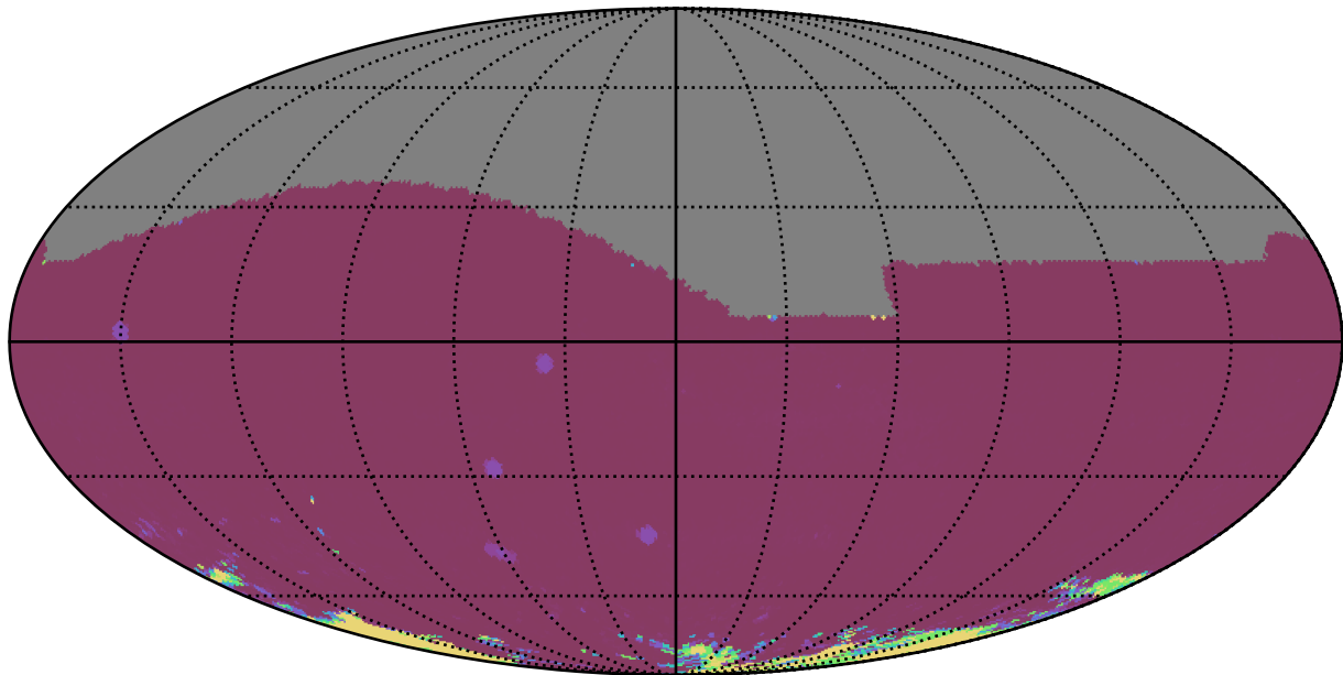
ddf_acor_sf20_lsf30_lsr10_v3.4_10yrs All sky iz bands: 75th Percentile Intranight Timespan
