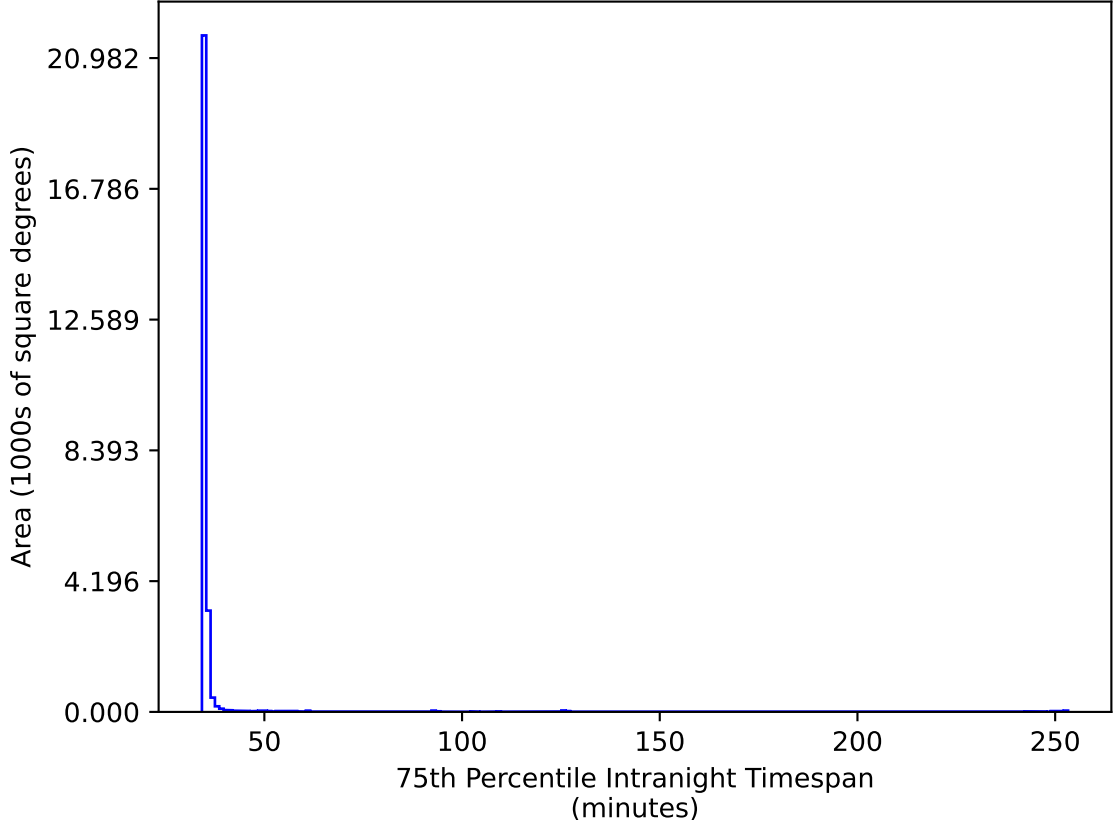
ddf_acor_sf20_lsf30_lsr10_v3.4_10yrs All sky gr bands: 75th Percentile Intranight Timespan
