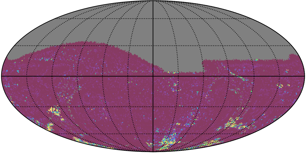
ddf_acor_sf20_lsf30_lsr10_v3.4_10yrs All sky g band: 75th Percentile Intranight Timespan
