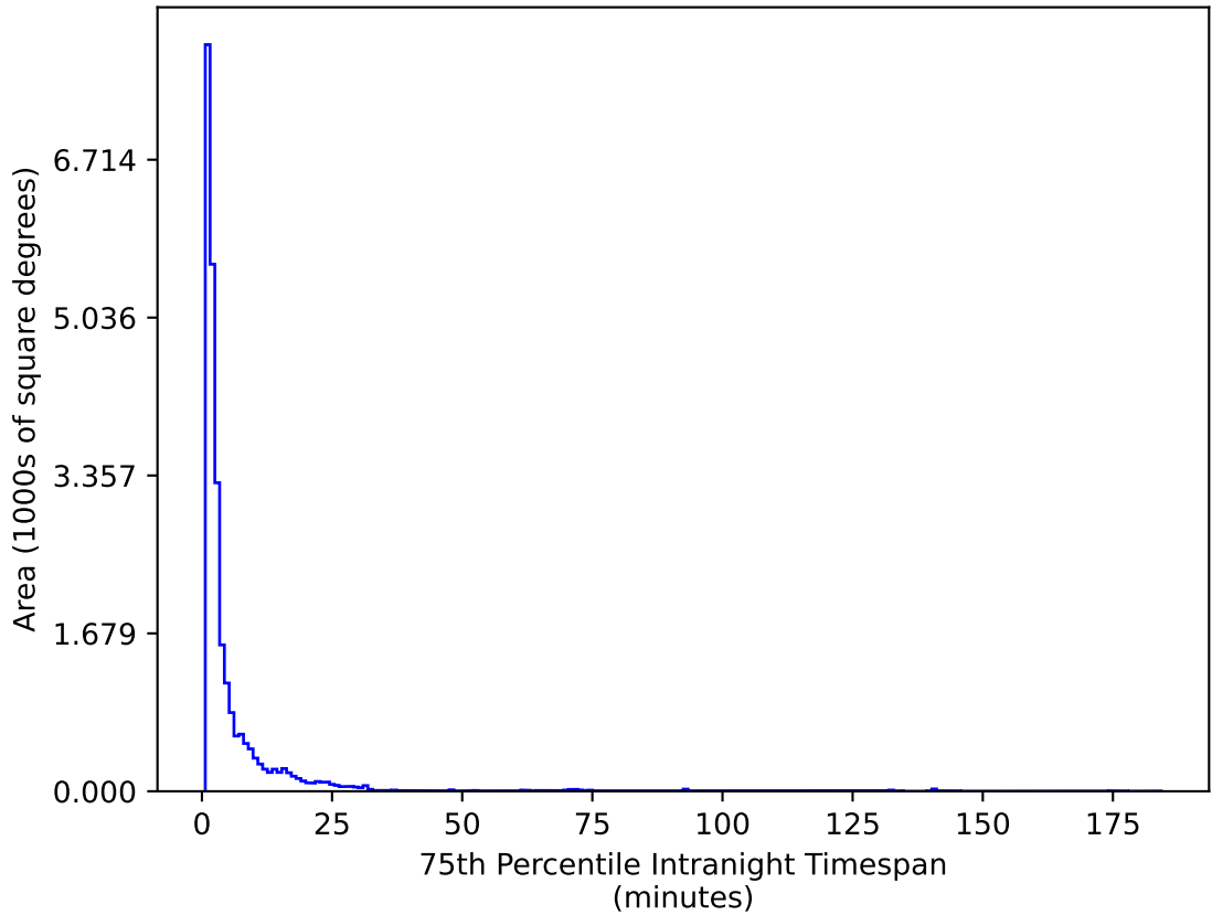
ddf_acor_sf20_lsf30_lsr10_v3.4_10yrs All sky g band: 75th Percentile Intranight Timespan
