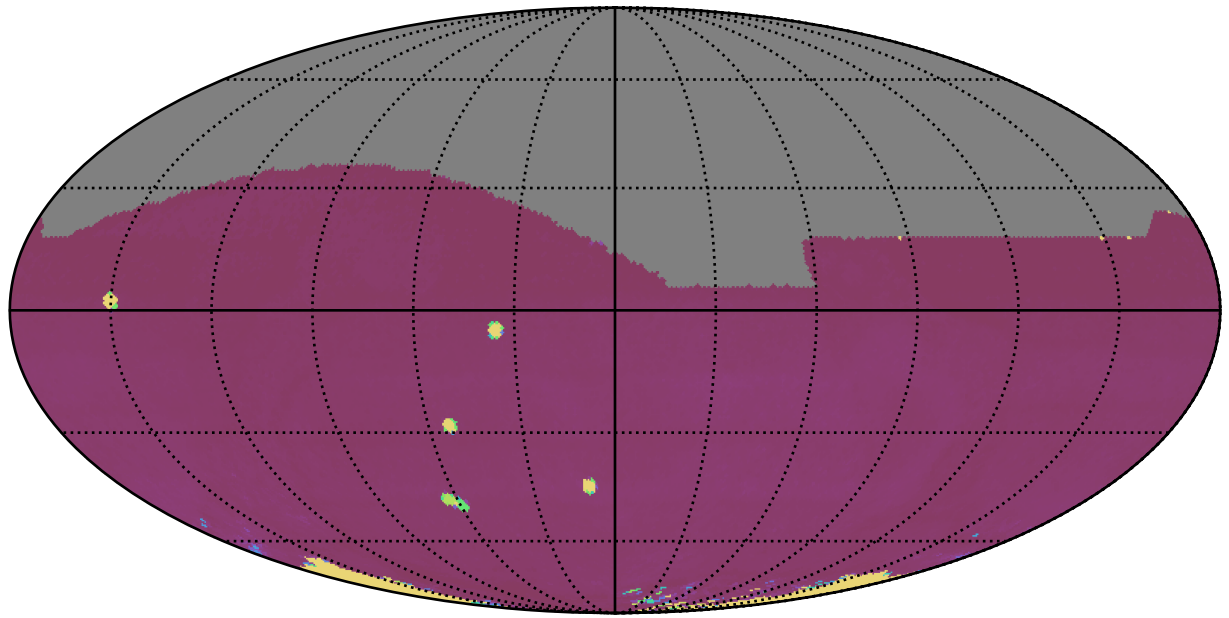
ddf_acor_sf20_lsf30_lsr10_v3.4_10yrs All sky: 75th Percentile Intranight Timespan
