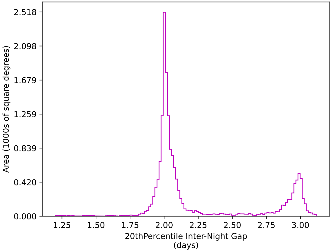
ddf_acor_sf20_lsf30_lsr10_v3.4_10yrs WFD z band: 20thPercentile Inter-Night Gap
