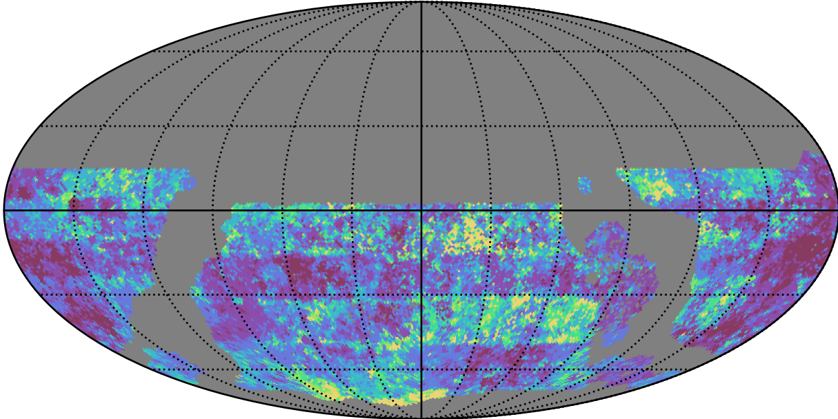
ddf_acor_sf20_lsf30_lsr10_v3.4_10yrs WFD g band: 20thPercentile Inter-Night Gap
