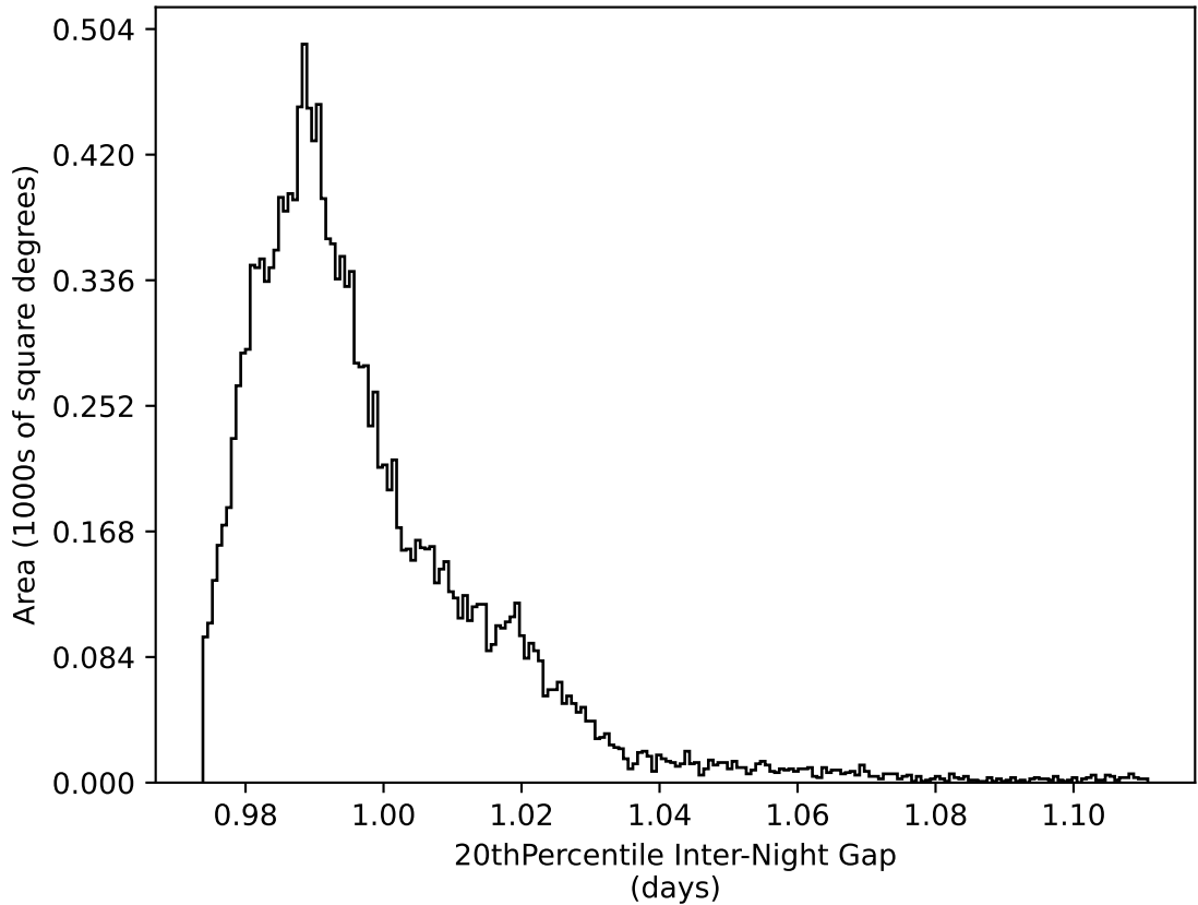
ddf_acor_sf20_lsf30_lsr10_v3.4_10yrs WFD all bands: 20thPercentile Inter-Night Gap
