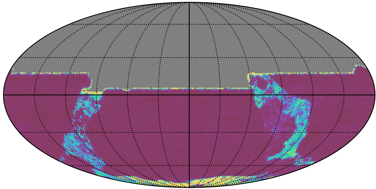
ddf_acor_sf20_lsf30_lsr10_v3.4_10yrs All sky y band: 20thPercentile Inter-Night Gap
