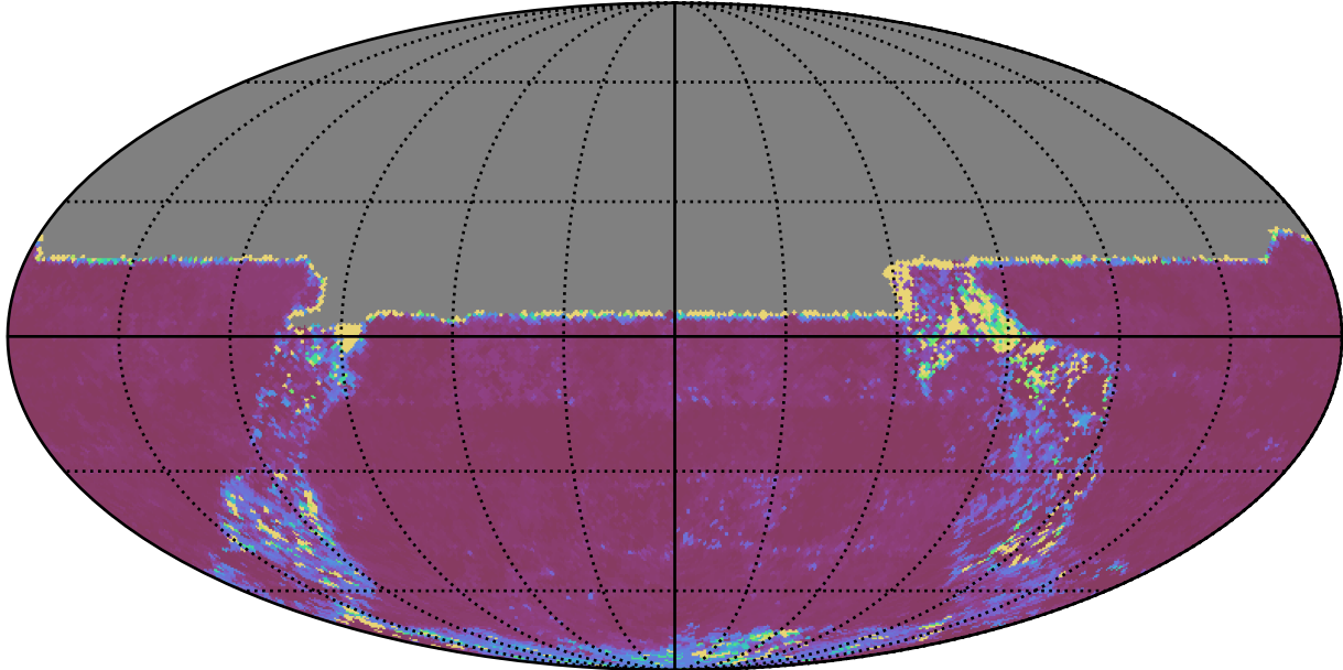
ddf_acor_sf20_lsf30_lsr10_v3.4_10yrs All sky u band: 20thPercentile Inter-Night Gap
