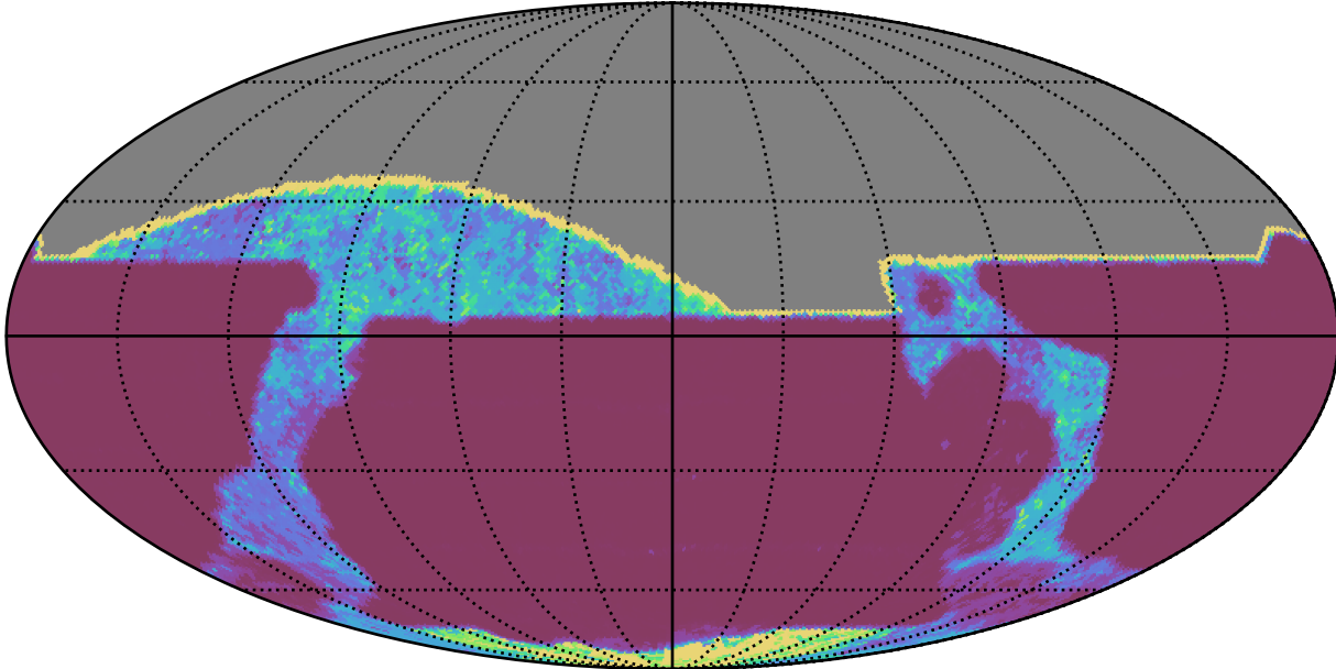
ddf_acor_sf20_lsf30_lsr10_v3.4_10yrs All sky all bands: 20thPercentile Inter-Night Gap
