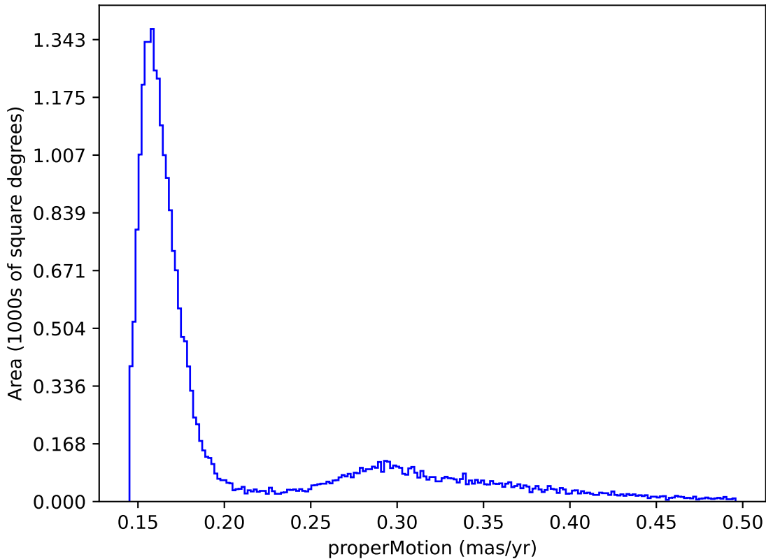
ddf_acor_sf20_lsf30_lsr10_v3.4_10yrs : properMotion
