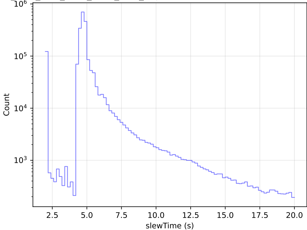
ddf_acor_sf20_Isf30_Isr10_v3.4_10yrs All visits: Zoom Slew Time Histogram
