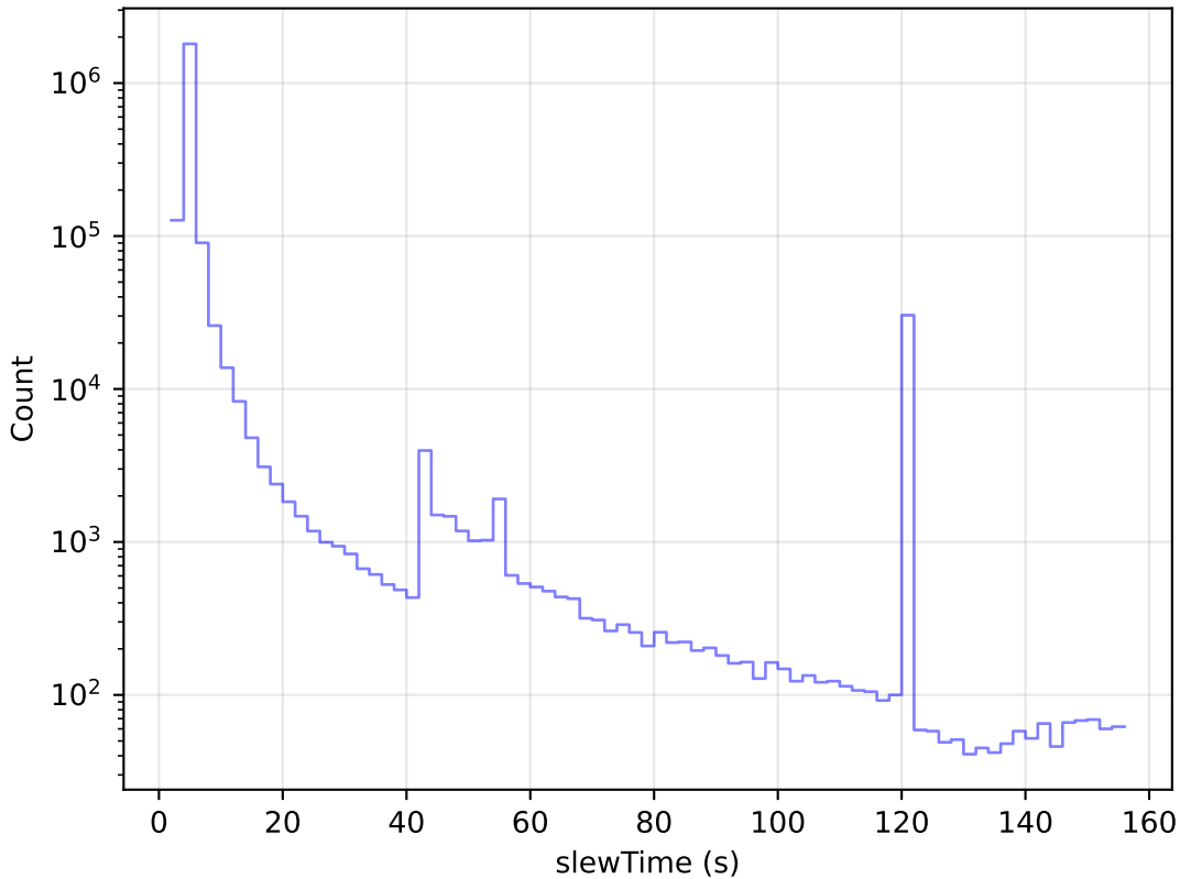
ddf_acor_sf20_lsf30_lsr10_v3.4_10yrs All visits: Slew Time Histogram
