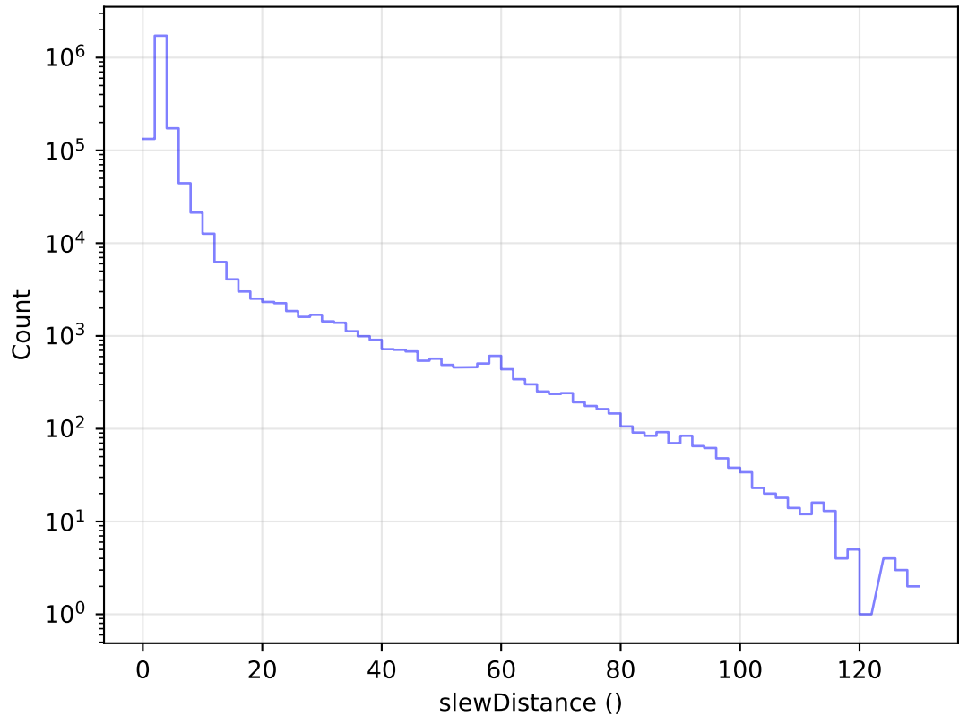
ddf_acor_sf20_lsf30_lsr10_v3.4_10yrs All visits: Slew Distance Histogram
