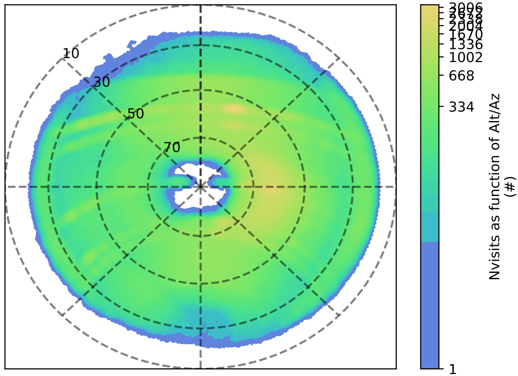
ddf_acor_sf20_lsf30_lsr10_v3.4_10yrs z: Nvisits as function of Alt/Az
