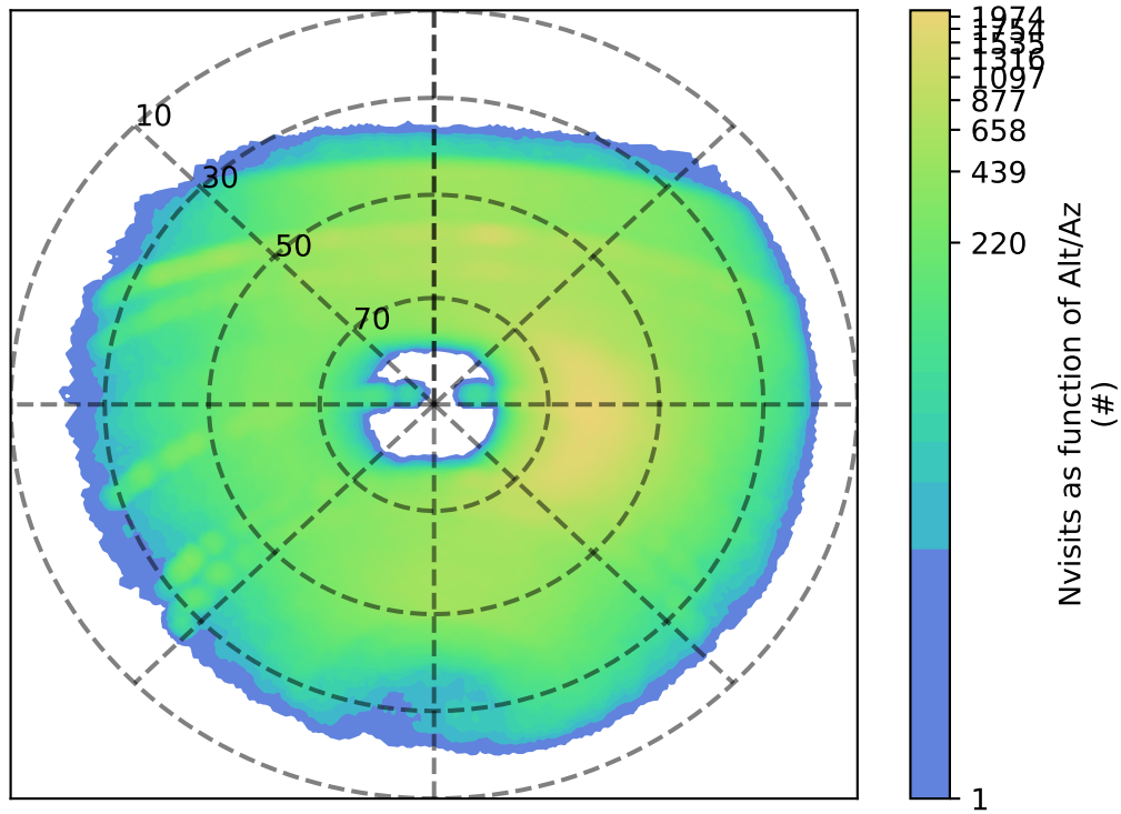
ddf_acor_sf20_lsf30_lsr10_v3.4_10yrs y: Nvisits as function of Alt/Az
