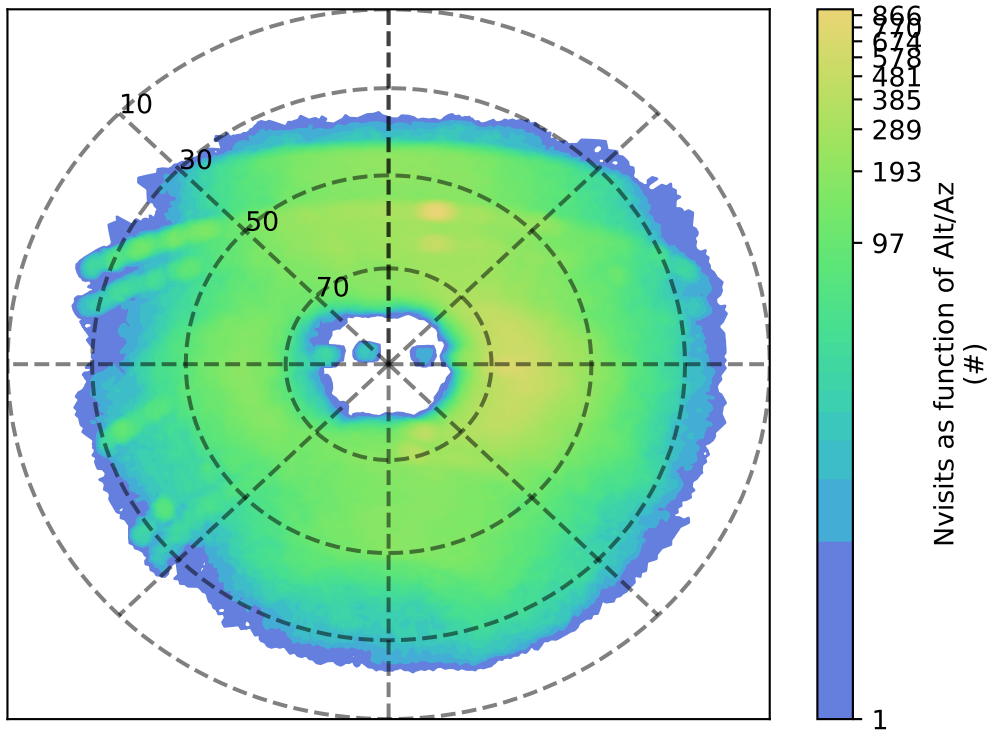
ddf_acor_sf20_ls30_lsr10_v3.4_10yrs u: Nvisits as function of Alt/Az
