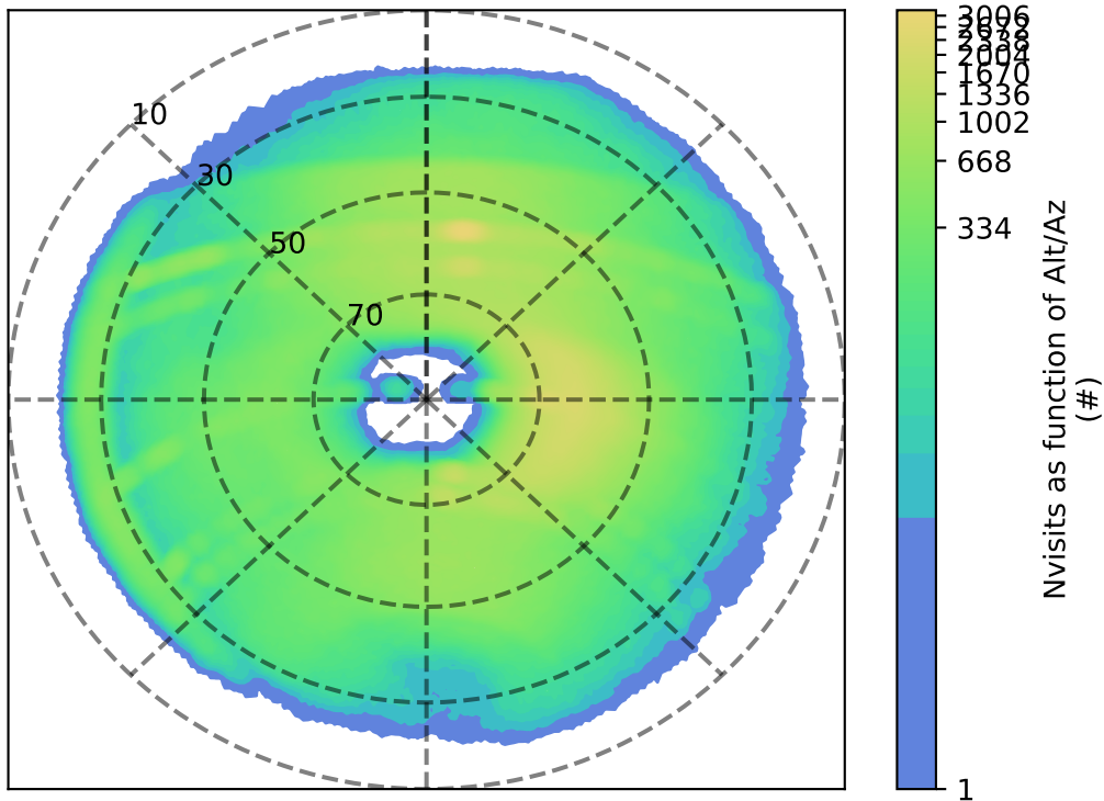
ddf_acor_sf20_lsf30_lsr10_v3.4_10yrs r: Nvisits as function of Alt/Az
