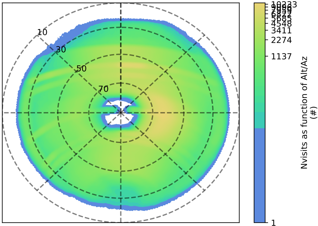
ddf_acor_sf20_lsf30_lsr10_v3.4_10yrs : Nvisits as function of Alt/Az
