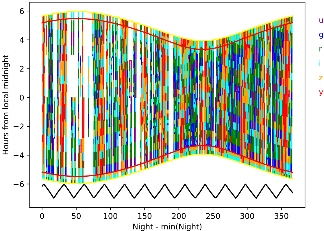
ddf_acor_sf20_lsf30_lsr10_v3.4_10yrs year 9-10: Hourglass
