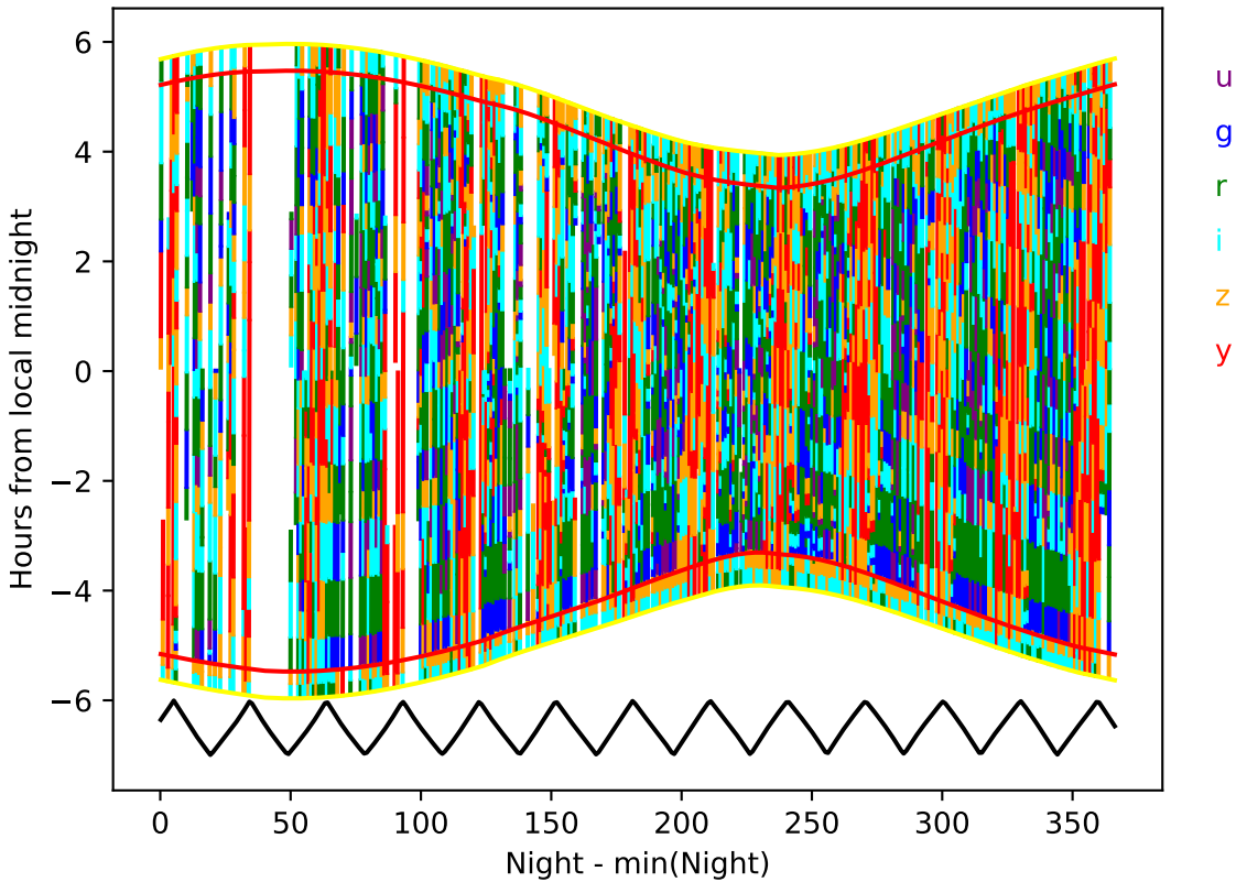
ddf_acor_sf20_lsf30_lsr10_v3.4_10yrs year 6-7: Hourglass
