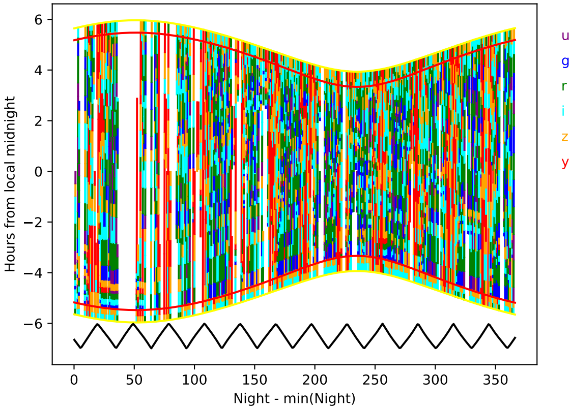
ddf_acor_sf20_lsf30_lsr10_v3.4_10yrs year 2-3: Hourglass
