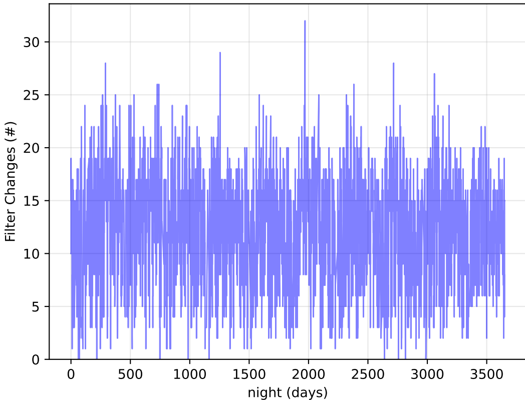
ddf_acor_sf20_lsf30_lsr10_v3.4_10yrs : Filter Changes
