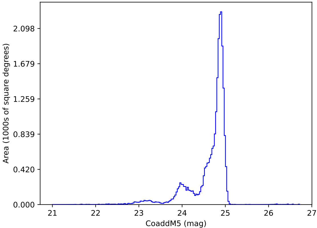
ddf_acor_sf20_lsf30_lsr10_v3.4_10yrs y: CoaddM5
