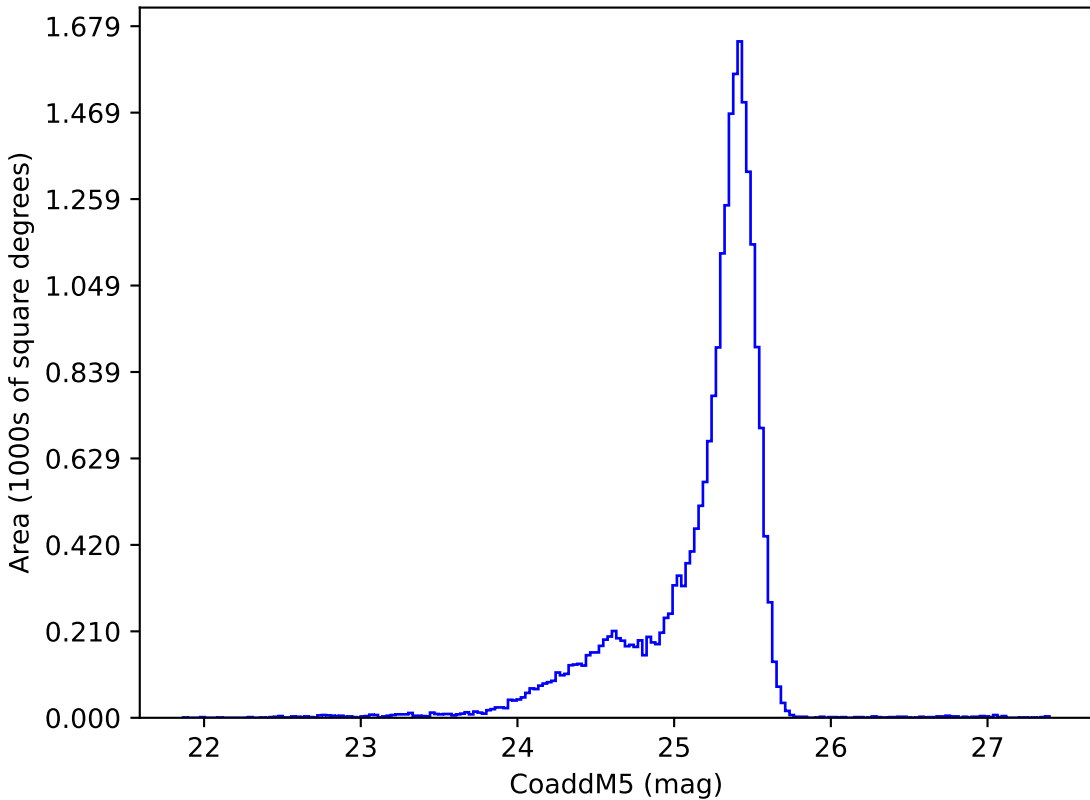
ddf_acor_sf20_lsf30_lsr10_v3.4_10yrs u: CoaddM5
