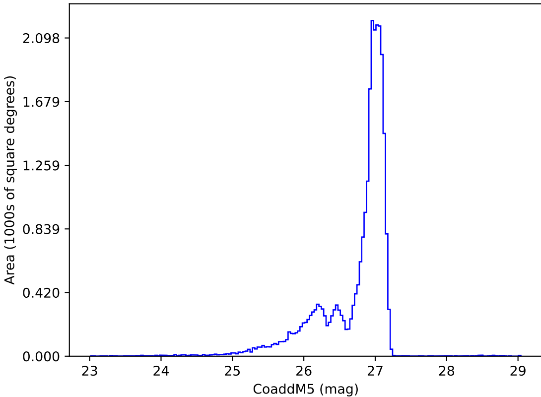
ddf_acor_sf20_lsf30_lsr10_v3.4_10yrs r: CoaddM5
