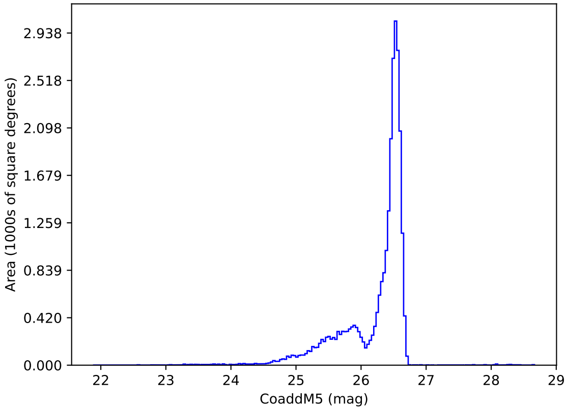
ddf_acor_sf20_lsf30_lsr10_v3.4_10yrs i: CoaddM5
