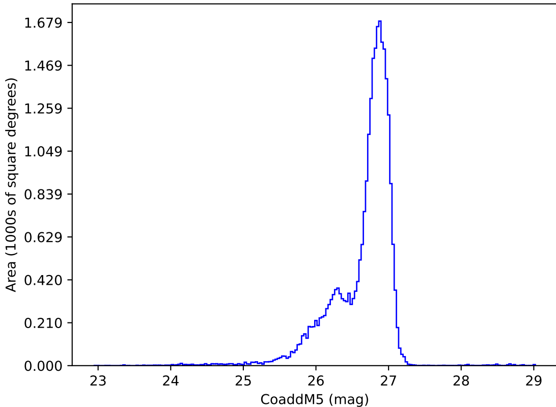
ddf_acor_sf20_lsf30_lsr10_v3.4_10yrs g: CoaddM5
