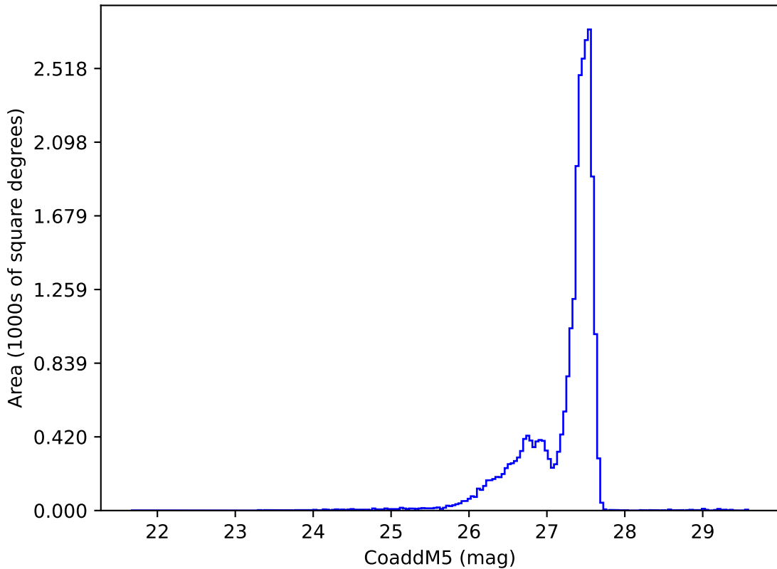
ddf_acor_sf20_lsf30_lsr10_v3.4_10yrs : CoaddM5
