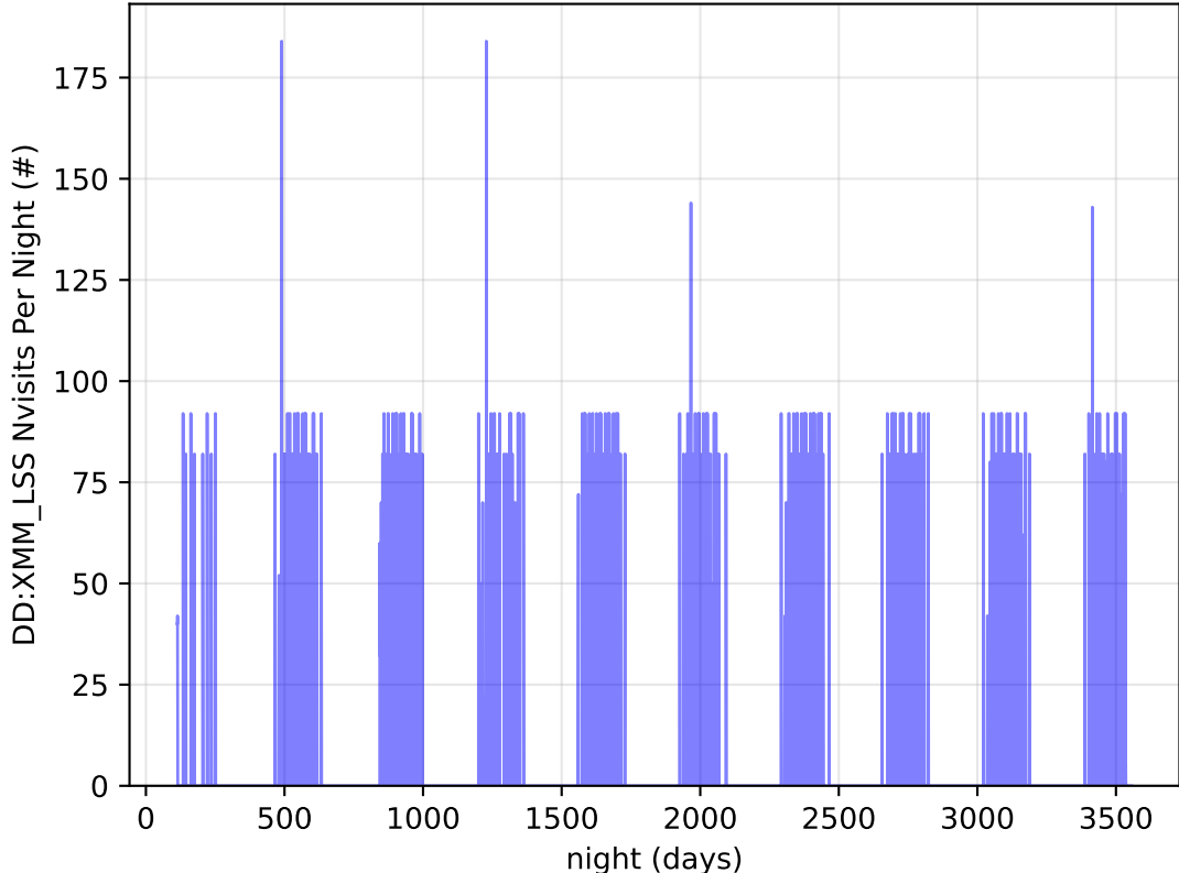
ddf_acor_sf20_lsf30_lsr10_v3.4_10yrs all bands: DD:XMM_LSS Nvisits Per Night
