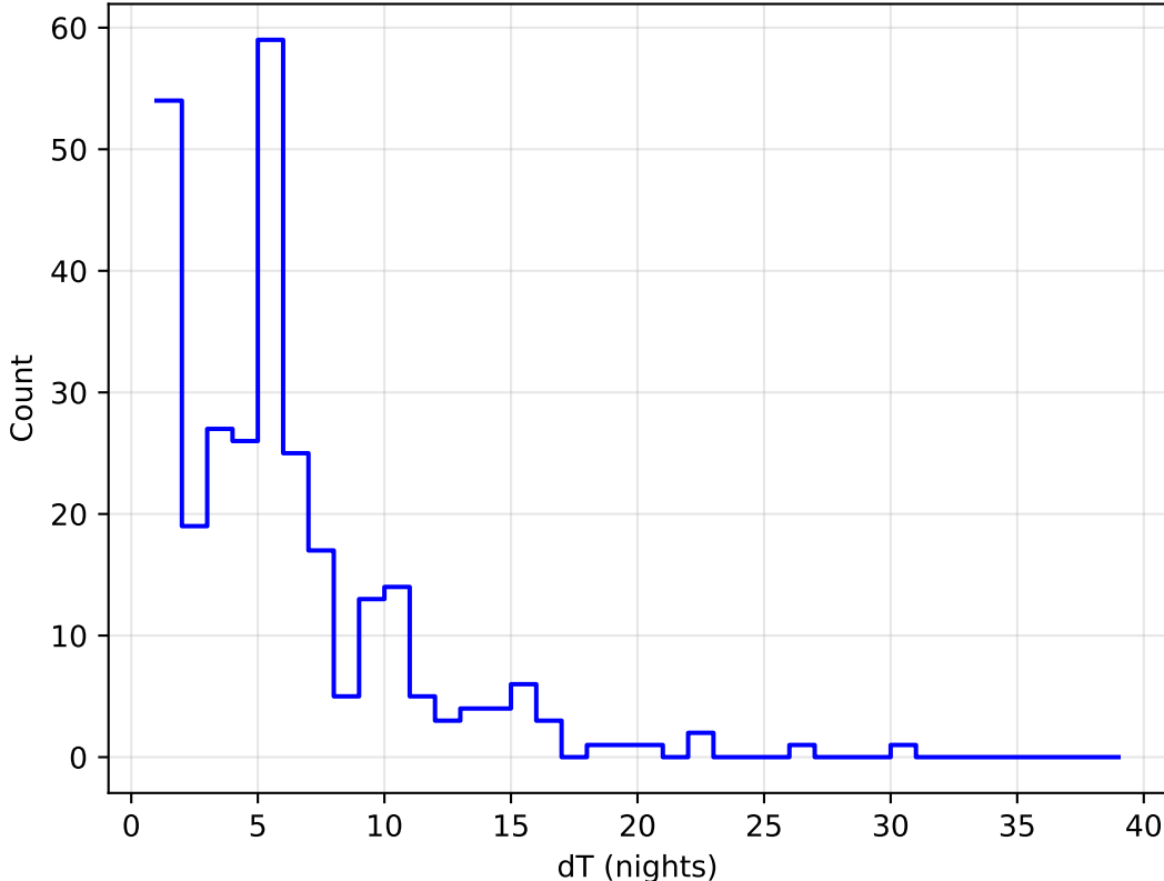
ddf_acor_sf20_Isf30_Isr10_v3.4_10yrs all bands: DD:XMM_LSS Delta Nights Histogram
