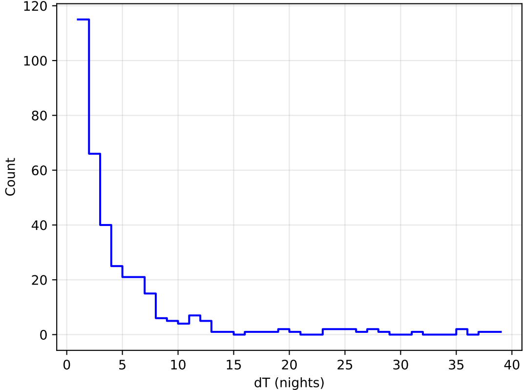
ddf_acor_sf20_lsf30_lsr10_v3.4_10yrs all bands: DD:WFD Delta Nights Histogram
