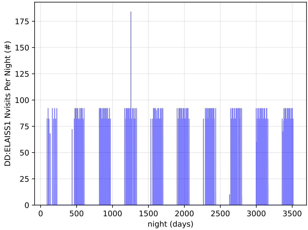
ddf_acor_sf20_lsf30_lsr10_v3.4_10yrs all bands: DD:ELAISS1 Nvisits Per Night
