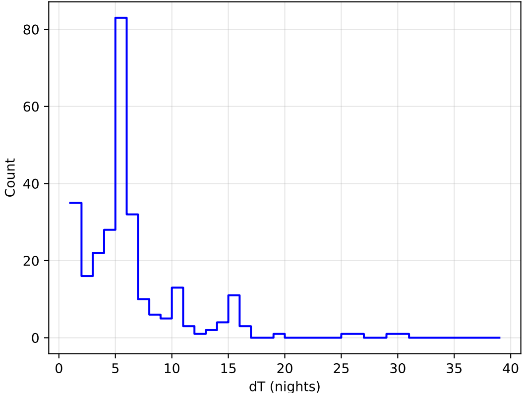
ddf_acor_sf20_lsf30_lsr10_v3.4_10yrs all bands: DD:ELAISS1 Delta Nights Histogram
