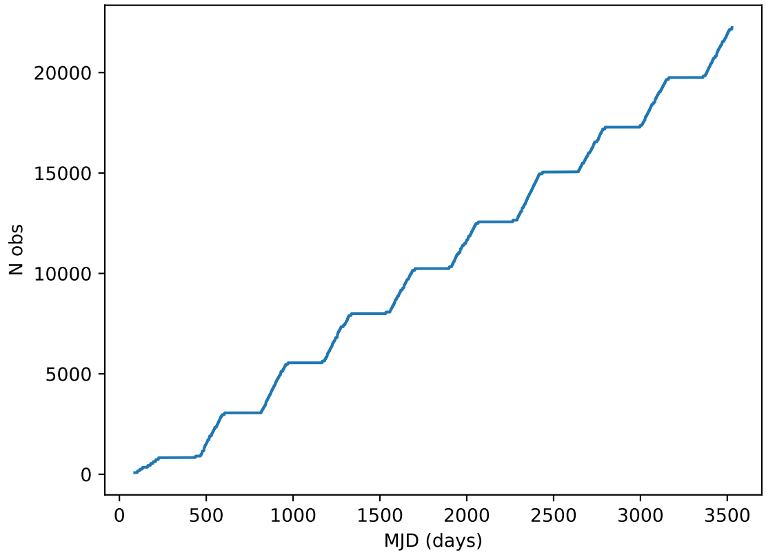
ddf_acor_sf20_lsf30_lsr10_v3.4_10yrs all bands: DD:ELAISS1 Cumulative NVisits
