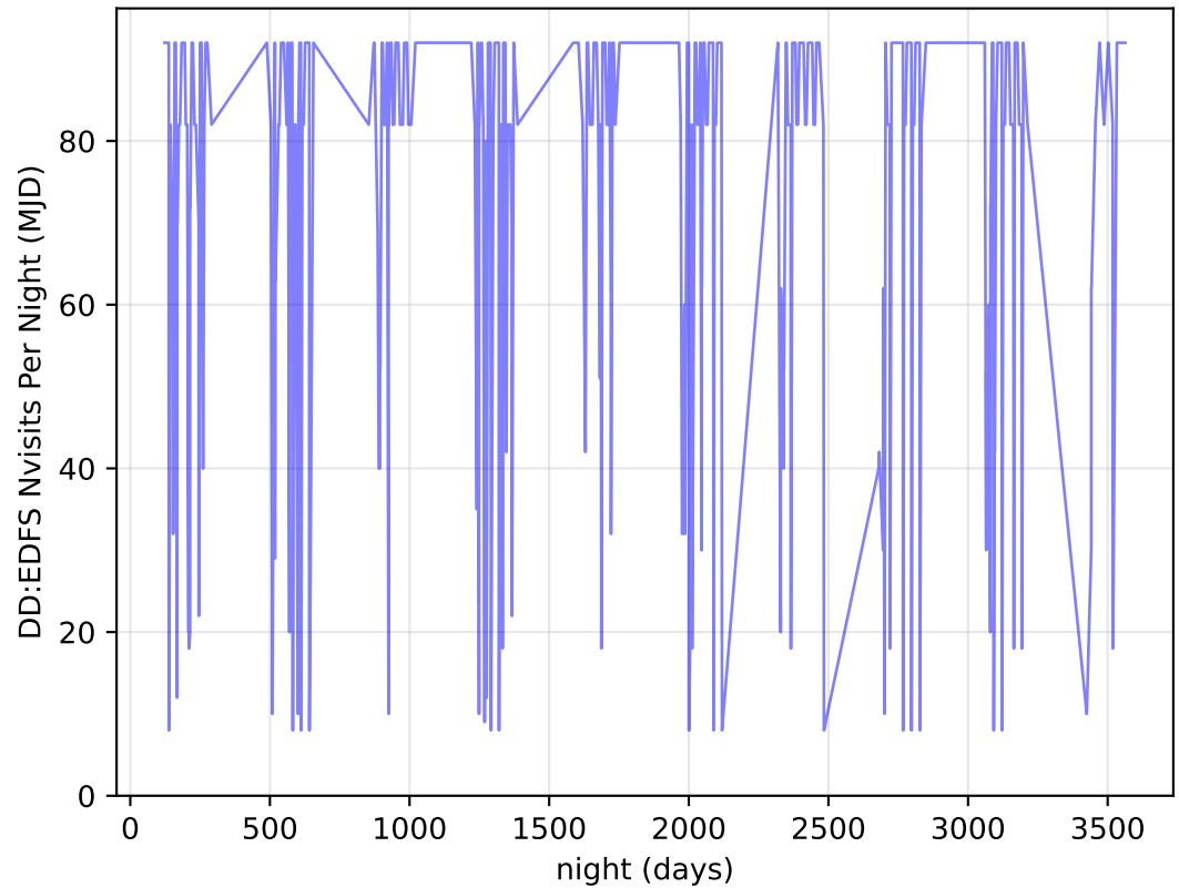
ddf_acor_sf20_lsf30_lsr10_v3.4_10yrs all bands: DD:EDFS Nvisits Per Night
