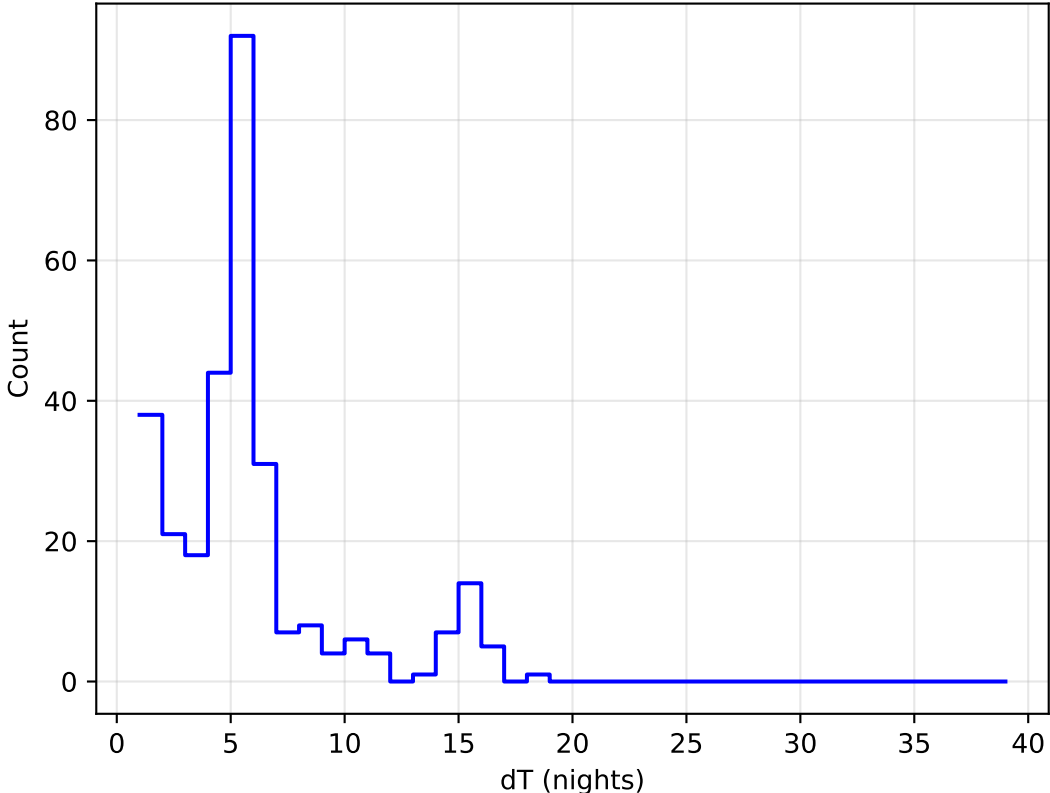
ddf_acor_sf20_lsf30_lsr10_v3.4_10yrs all bands: DD:EDFS Delta Nights Histogram
