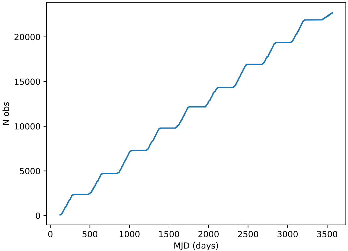
ddf_acor_sf20_lsf30_lsr10_v3.4_10yrs all bands: DD:EDFS Cumulative NVisits
